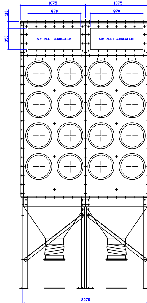
FRONT ELEVATION
