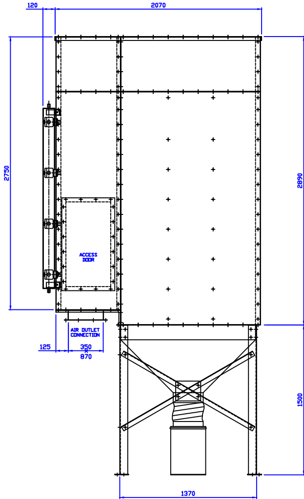
SIDE ELEVATION
