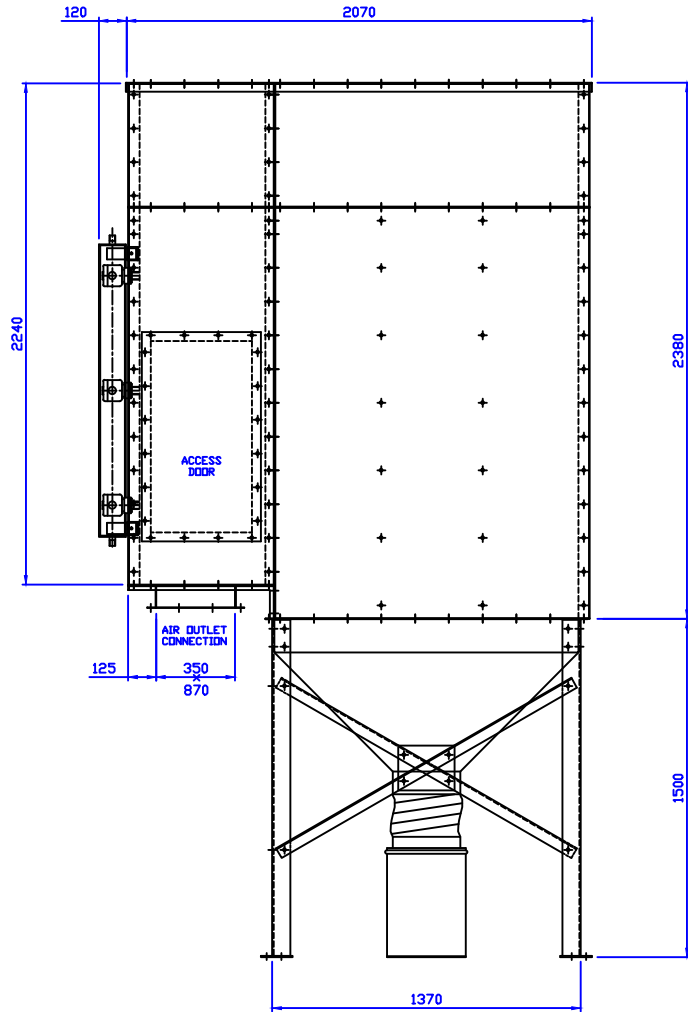
SIDE ELEVATION
